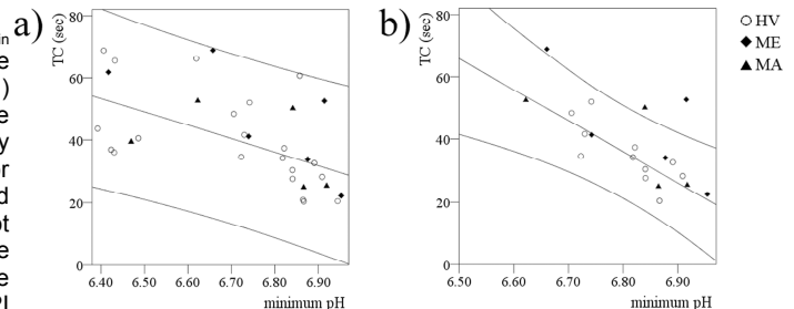
Figure 1: Phosphocreatine (PCr) recovery time plotted against minimum pH ( pH_{min} ) without exclusions in a) compared to with exclusions in b); equation for regression line and r value;
